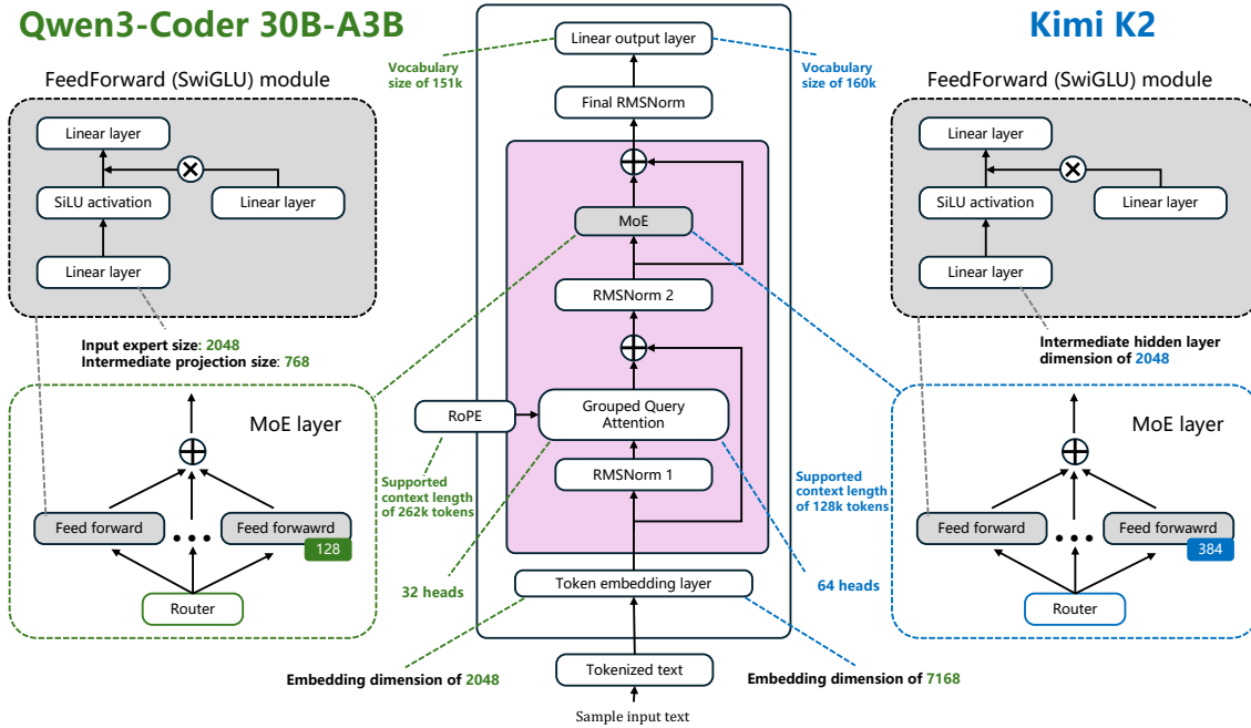
Figure 8. Architectural comparison between Kimi-K2-Instruct and Qwen3-Coder.
