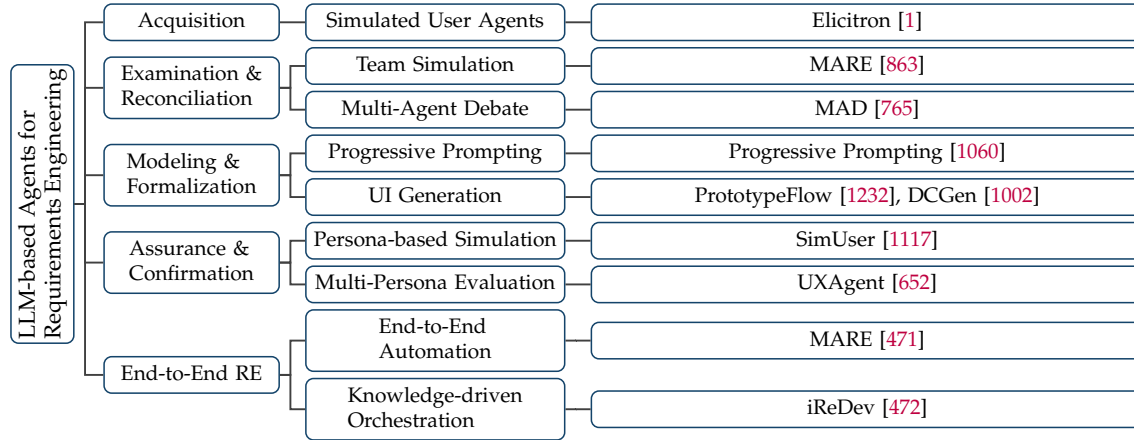
Figure 27. Taxonomy of LLM-based Agents for Requirements Engineering.
