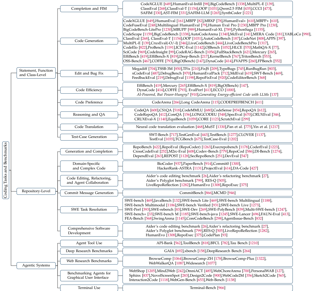
Figure 13. A Taxonomy of coding tasks and benchmarks.
