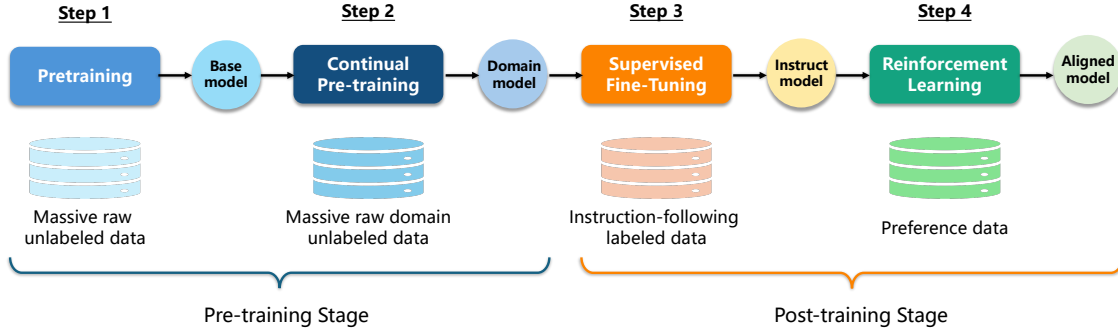
Figure 12. Overview of the model training stages.
