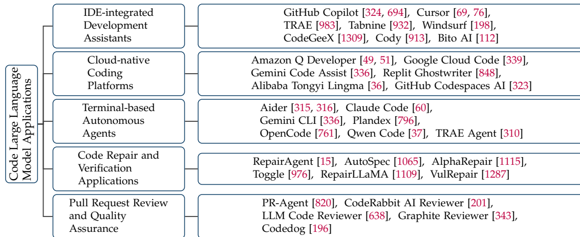
Figure 51. Code Large Language Model Applications.
