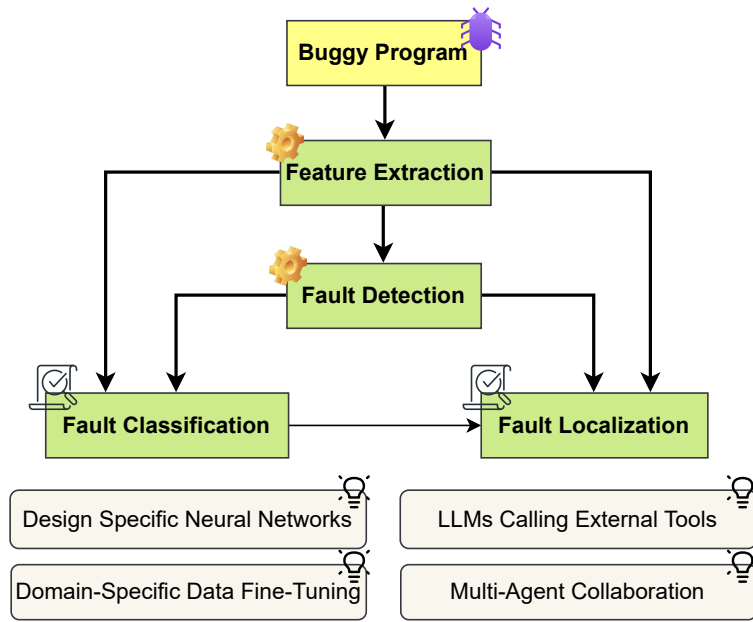
Figure 30. Taxonomy of End-to-end Fault Localization.
