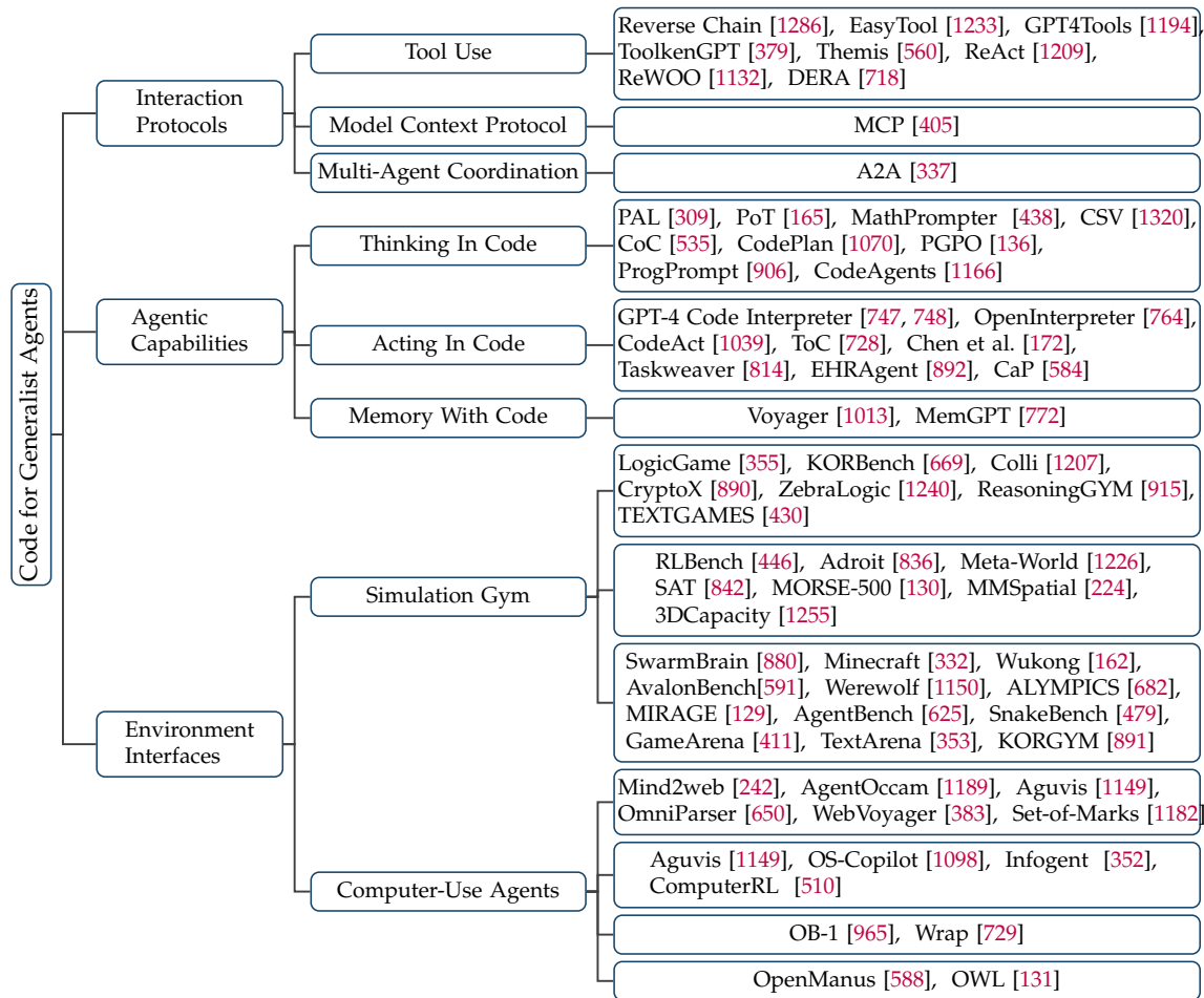
Figure 37. Taxonomy of Code for Generalist Agents.
