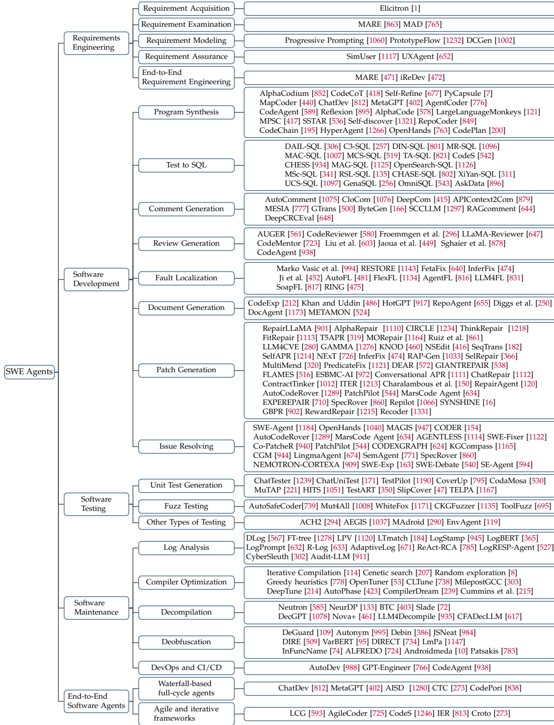
Figure 26. SWE-Agents in software engineering lifecycles.
