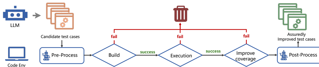
Figure 35. Overview of unit test generation.
