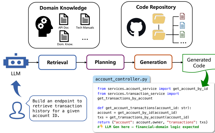
Figure 15. Illustration of the domain-specific and complex code generation task.
